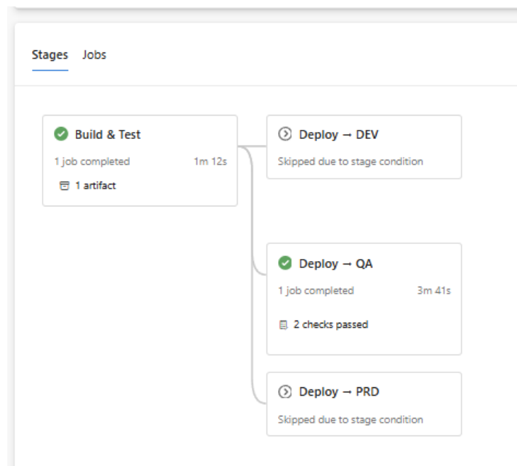
Figure 9: CI/CD Pipeline
