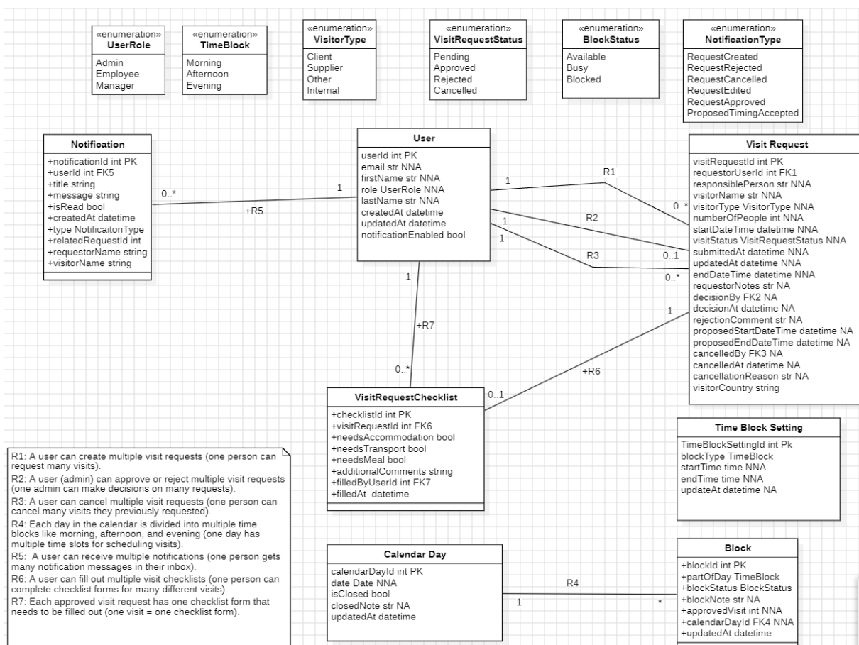
Figure 2: ERD Diagram
